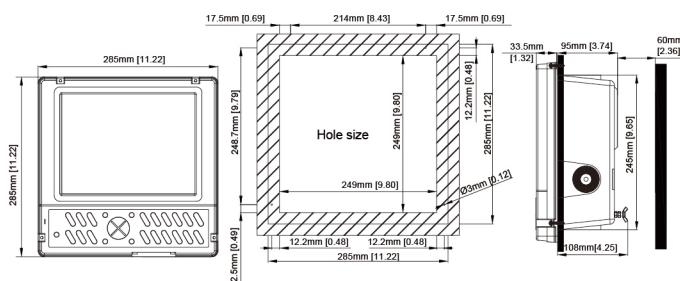
Flush mount
