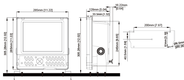
Bracket mount
