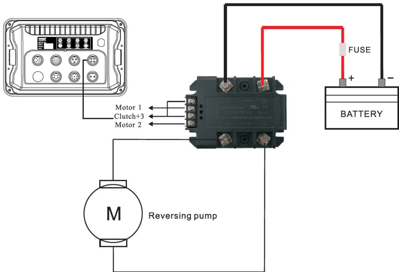
Connection with ONWA autopilot KAP-866
