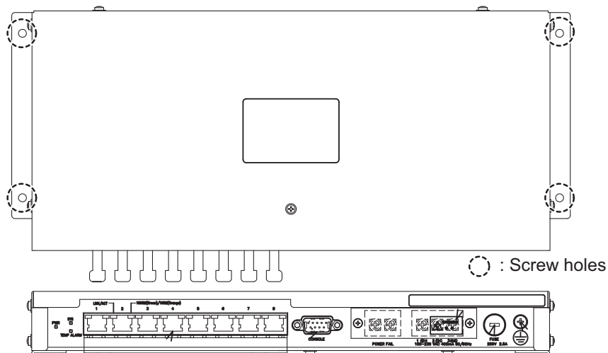
HUB-3000, bottom view
