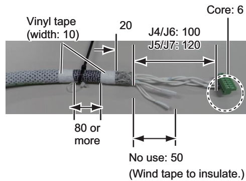
DPYC-1.5 cable
