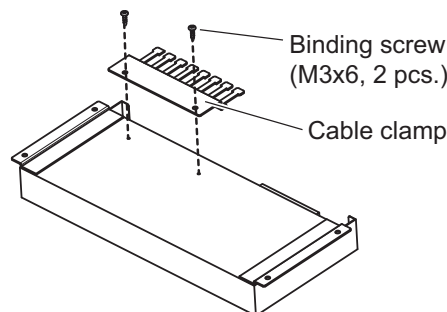
HUB-3000, bottom view
