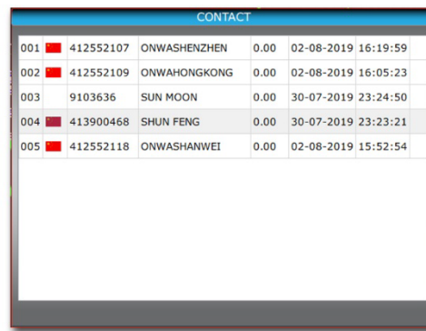
Chat History
