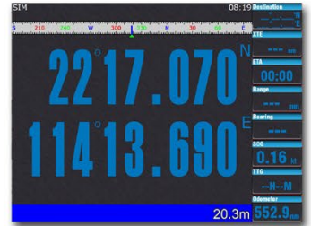
Navigation
